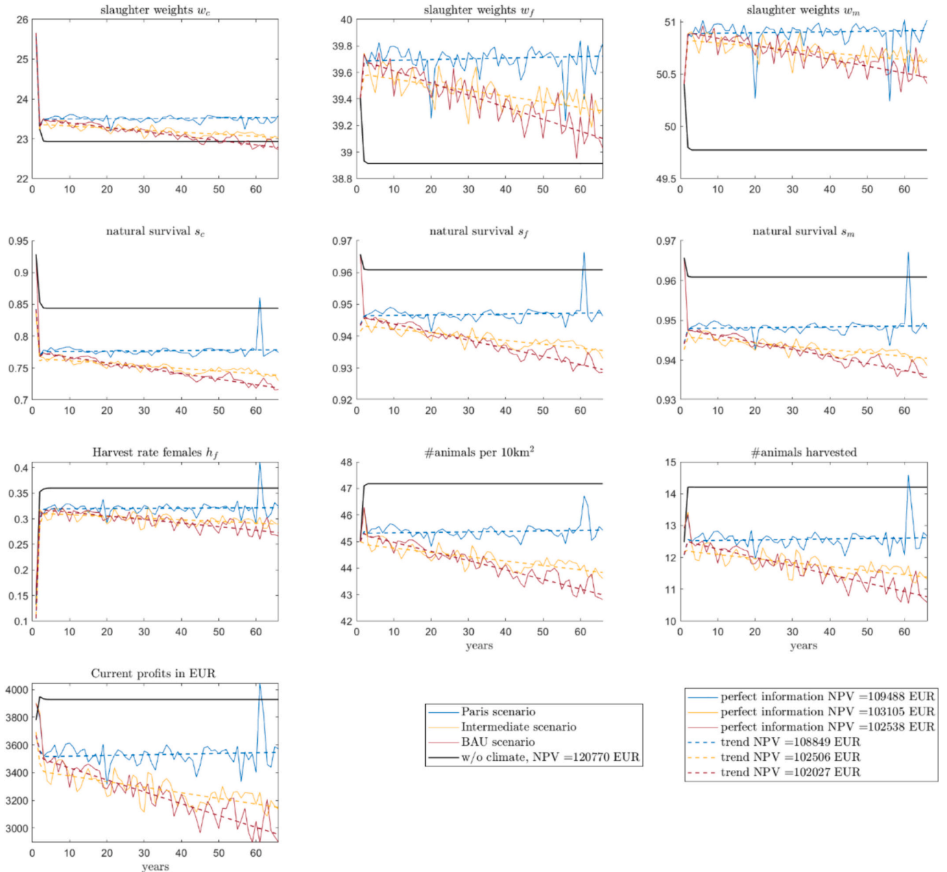
Fig. 5. Optimal paths for the perfect information and trend case for all climate change scenarios in north Sweden, baseline parameter values.
