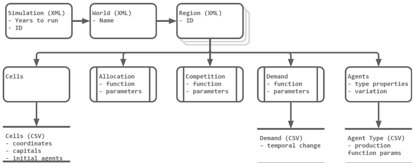
Fig. 3. Overview of the configuration of CRAFTY, showing relationships between files and what each file provides. CSV files provide basic data about cells, demand levels and agent production functions, and any temporal change in these, while XML files are used to identify these CSV files, to parameterise allocation, competition and demand functions, and to parameterise agent behaviour. An application of CRAFTY can therefore be set up using only the CSV and XML files shown here.
